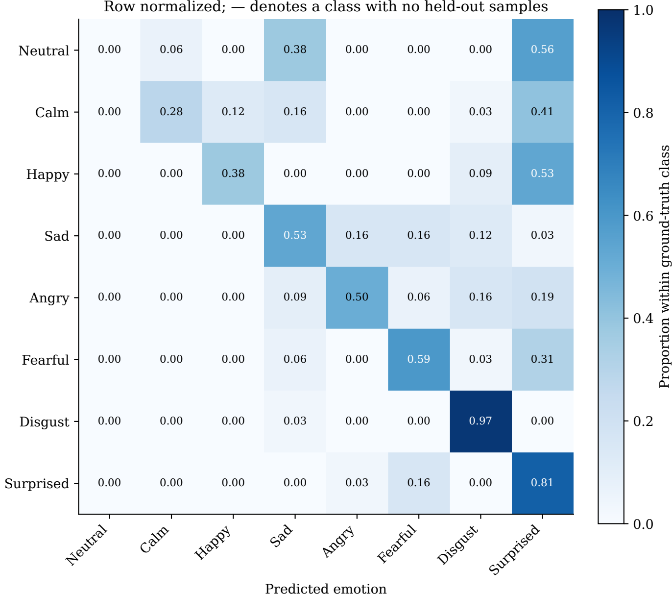
Adapted Intermediate Attention — Fold 1 | 6/6 folds Row normalized; — denotes a class with no held-out samples
