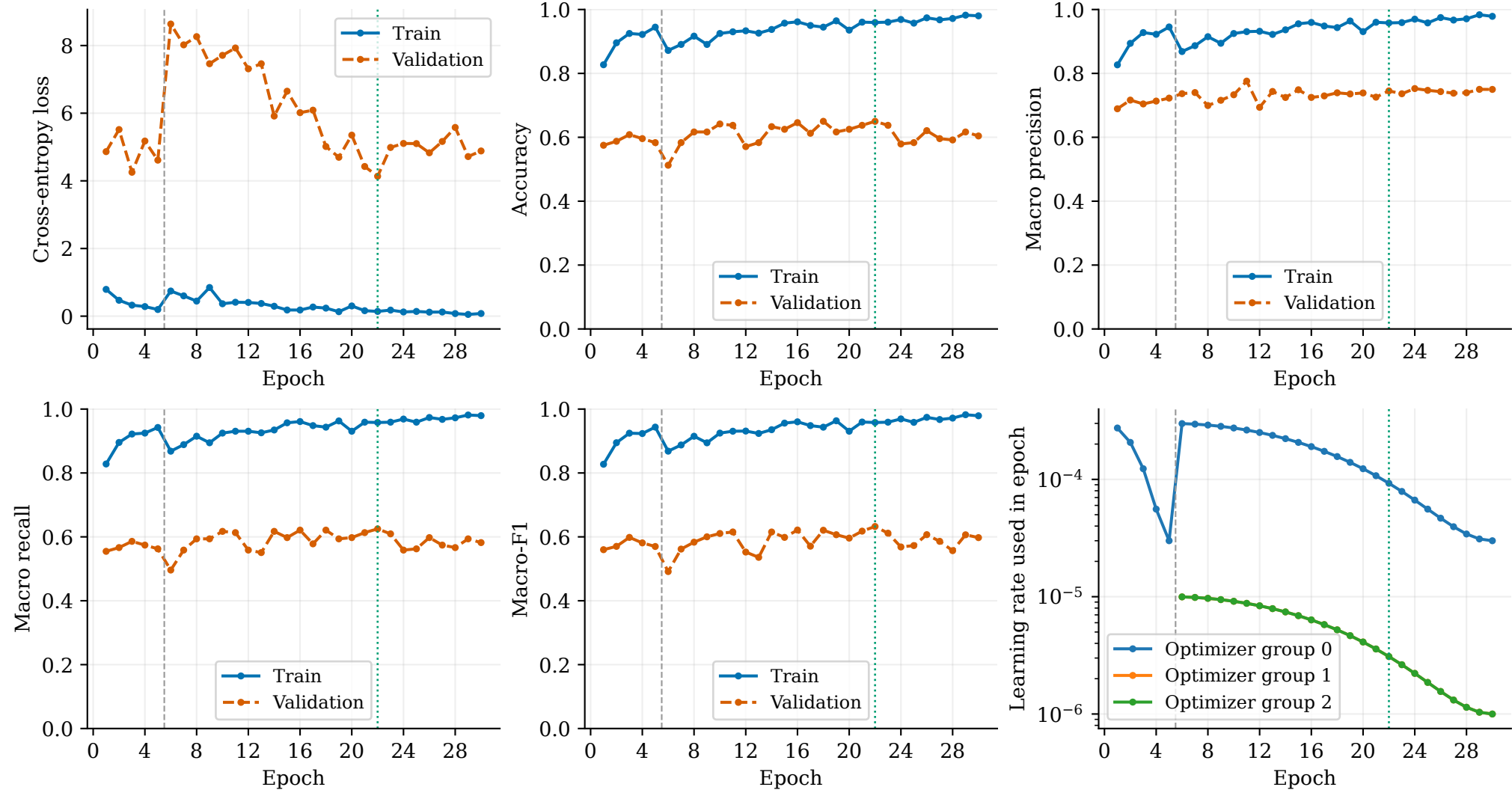
Adapted Intermediate Attention — Fold 1 | 6/6 folds Dotted green: best validation epoch; dashed gray: training stage change
