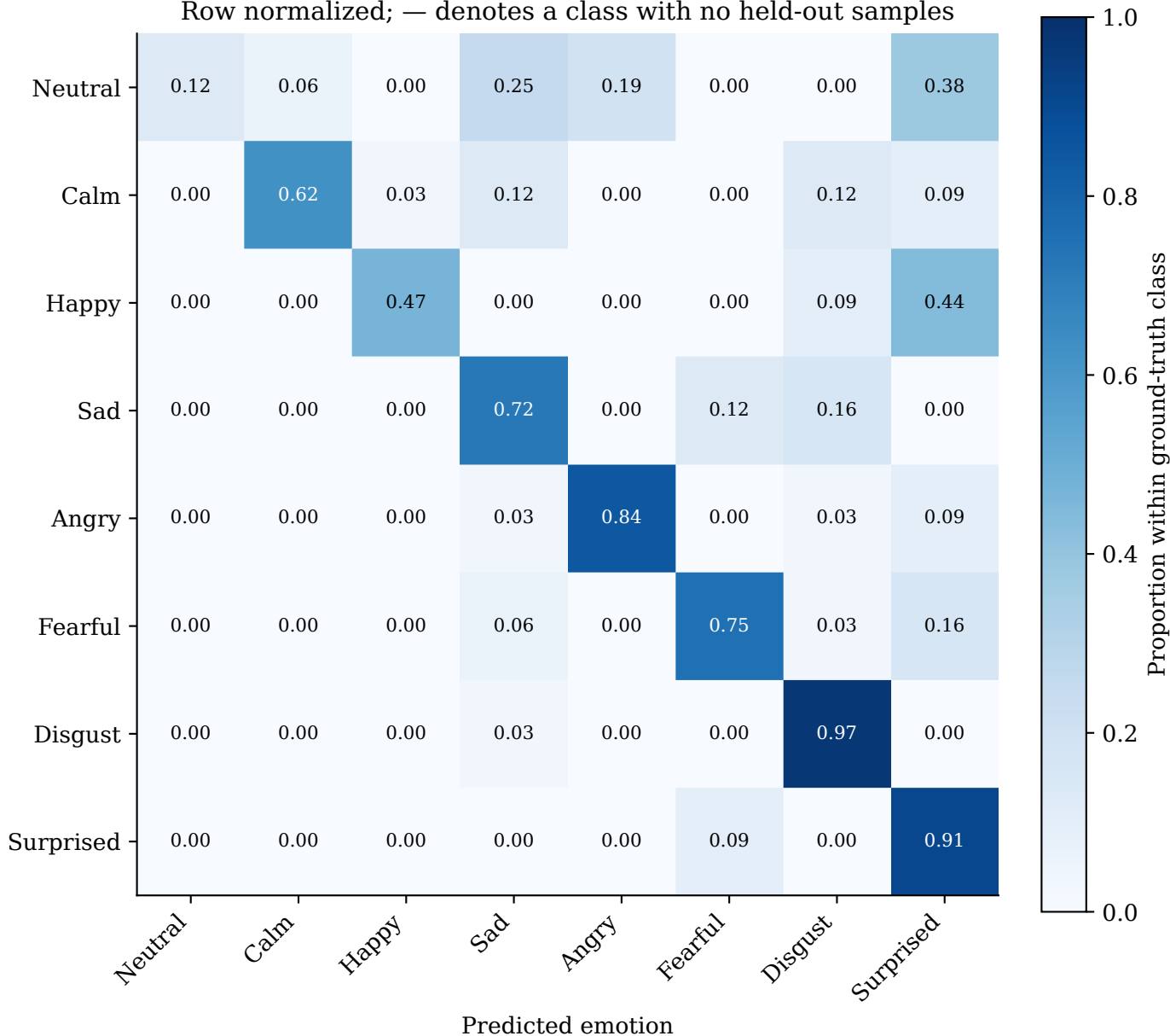
Cross-attention — Fold 1 | 6/6 folds Row normalized; — denotes a class with no held-out samples
