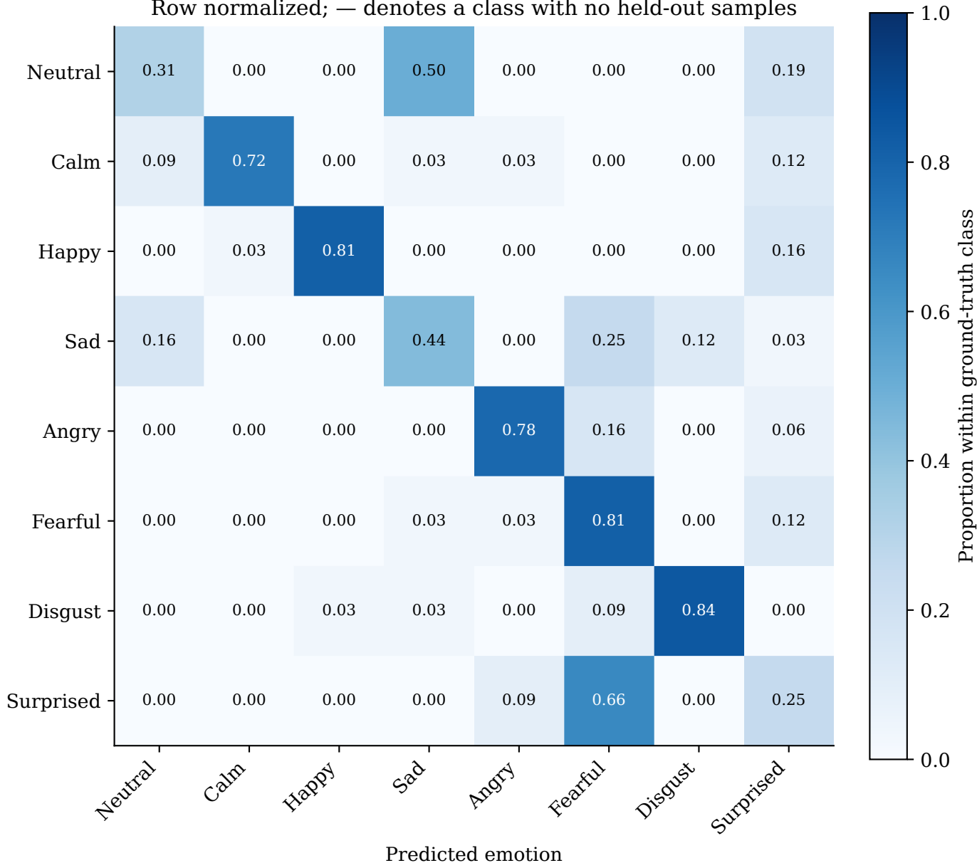
Video — Fold 2 | 6/6 folds Row normalized; — denotes a class with no held-out samples
