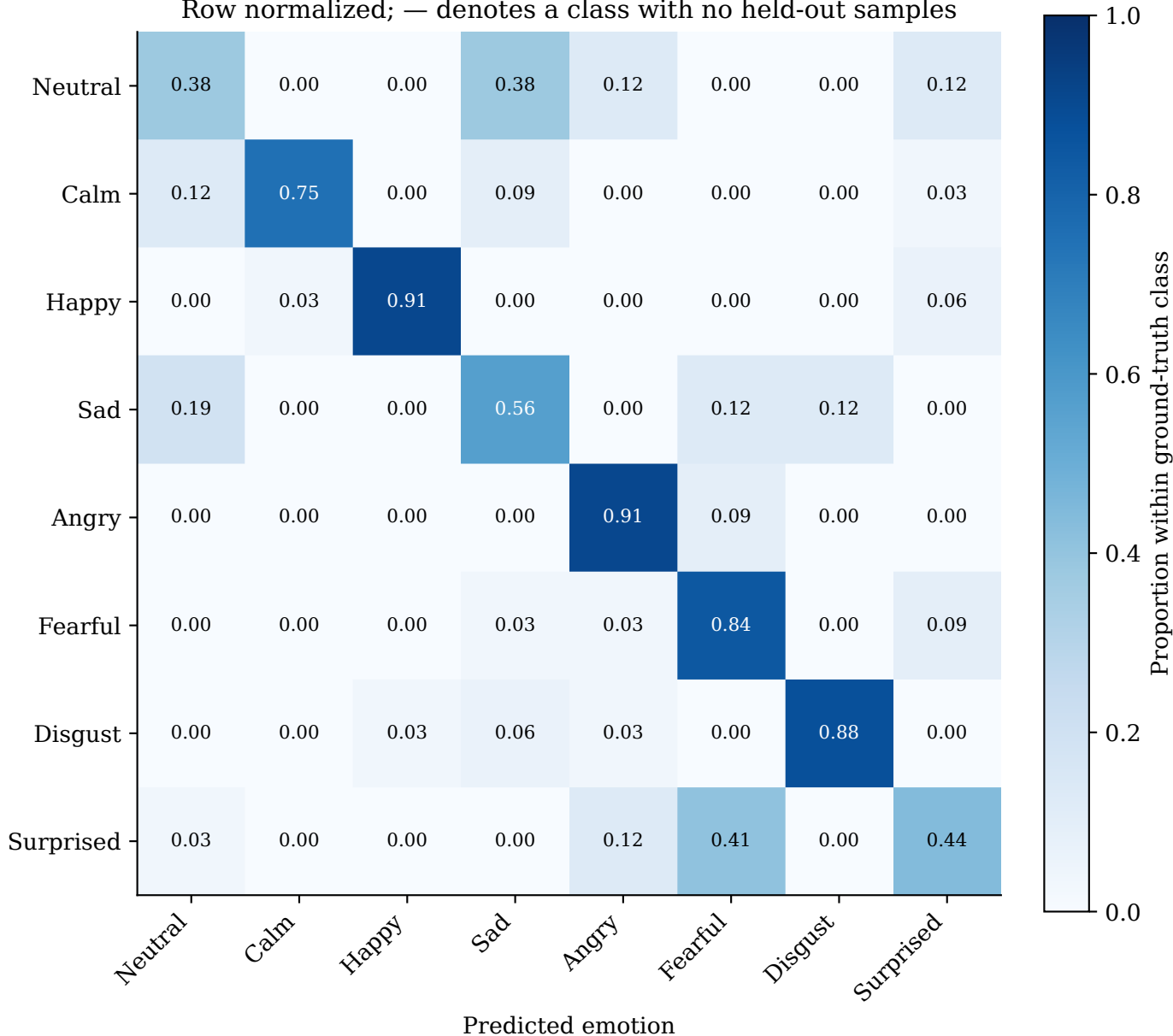
Cross-attention — Fold 2 | 6/6 folds Row normalized; — denotes a class with no held-out samples
