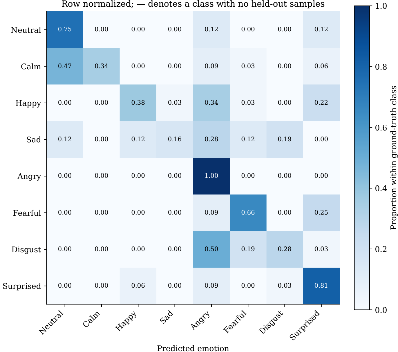
Audio — Fold 4 | 6/6 folds Row normalized; — denotes a class with no held-out samples
