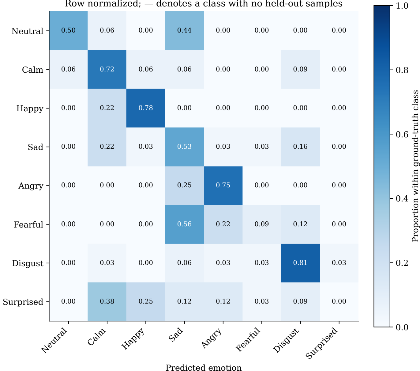
Video — Fold 4 | 6/6 folds Row normalized; — denotes a class with no held-out samples
