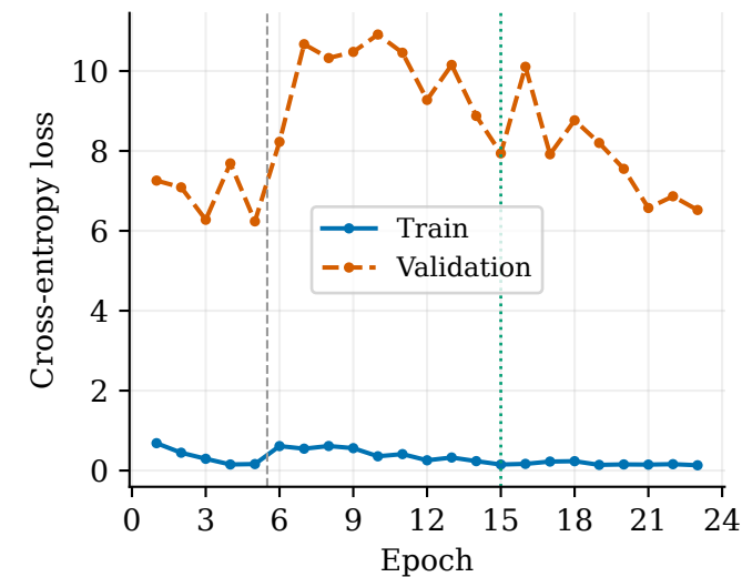
Adapted Intermediate Attention — Fold 5 | 6/6 folds Dotted green: best validation epoch; dashed gray: training stage change
