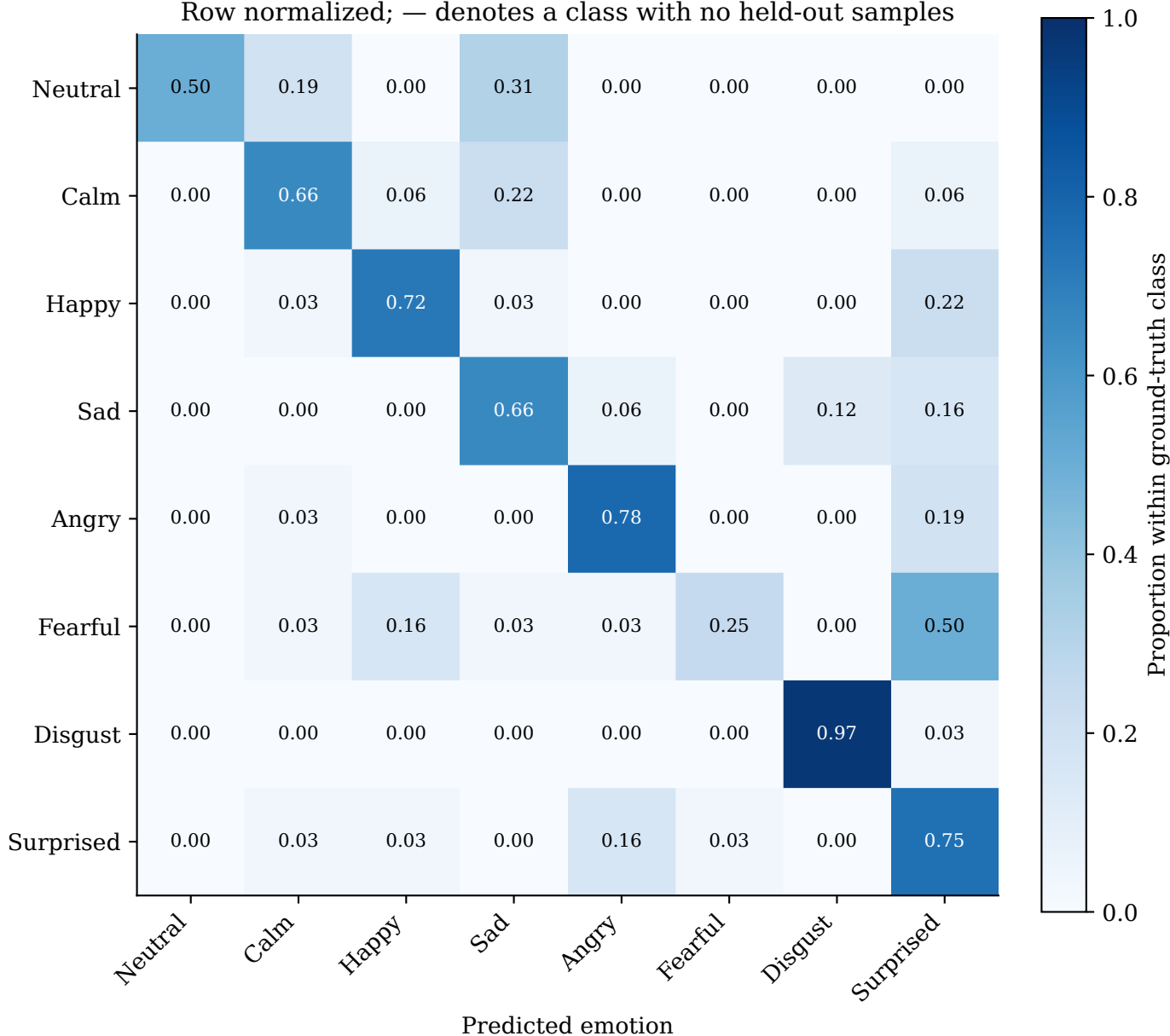
Gated fusion — Fold 5 | 6/6 folds Row normalized; — denotes a class with no held-out samples
