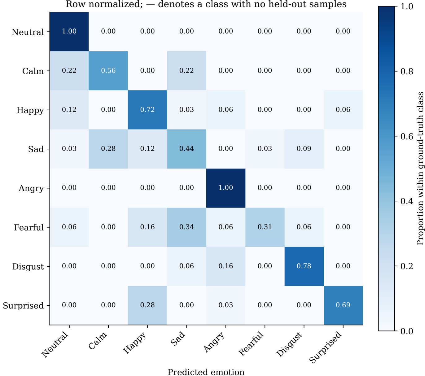
Audio — Fold 6 | 6/6 folds Row normalized; — denotes a class with no held-out samples
