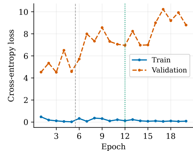
Adapted Intermediate Attention — Fold 6 | 6/6 folds Dotted green: best validation epoch; dashed gray: training stage change
