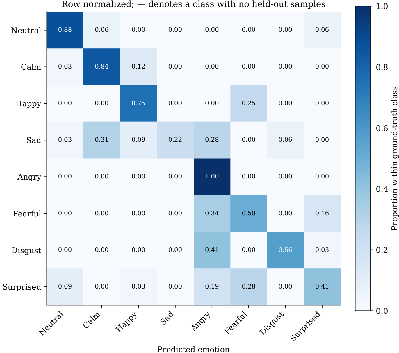
Gated fusion — Fold 6 | 6/6 folds Row normalized; — denotes a class with no held-out samples
