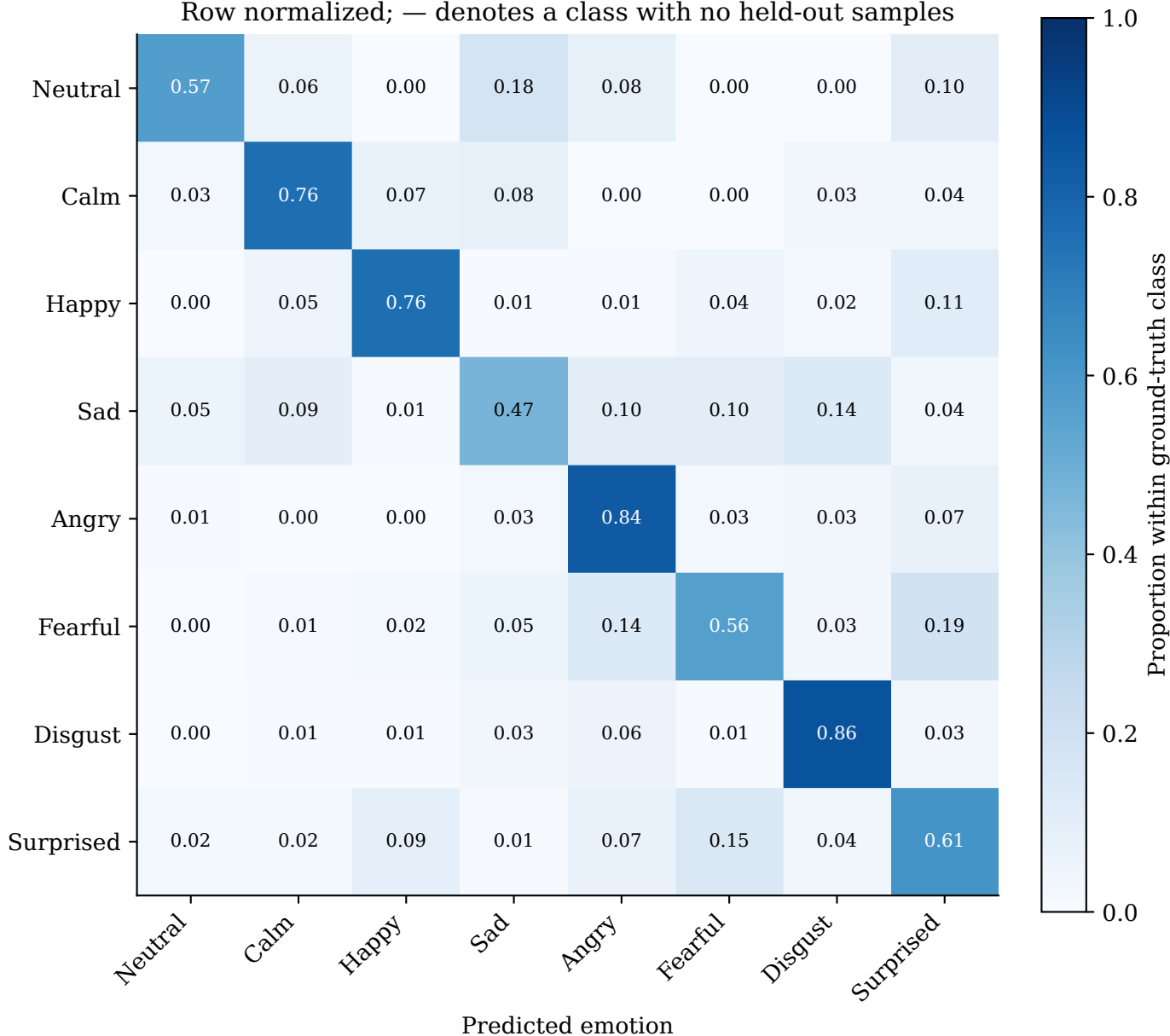
Cross-attention — pooled held-out predictions | 6/6 folds Row normalized; — denotes a class with no held-out samples
