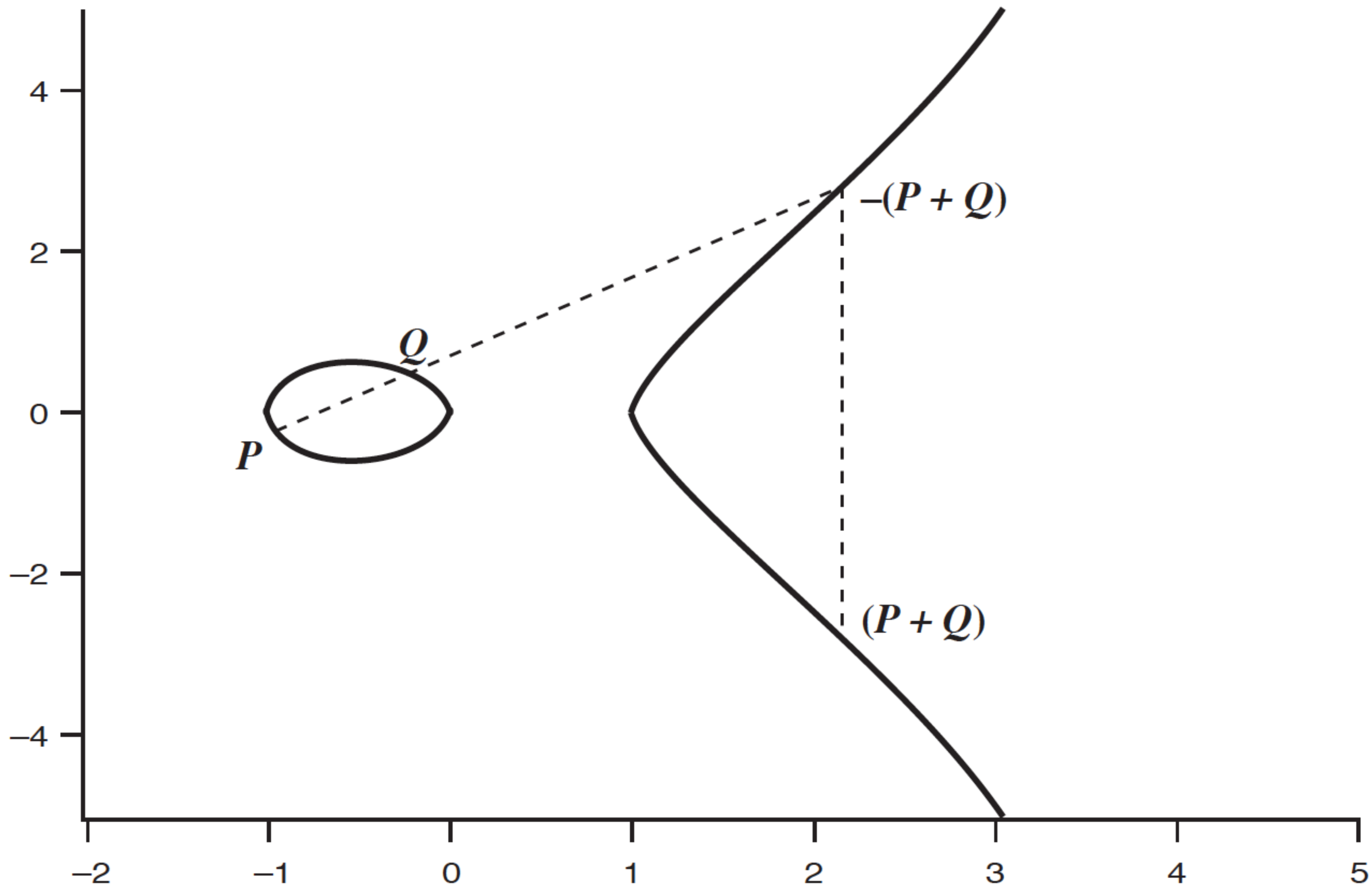
(a) y^2 = x^3 - x
