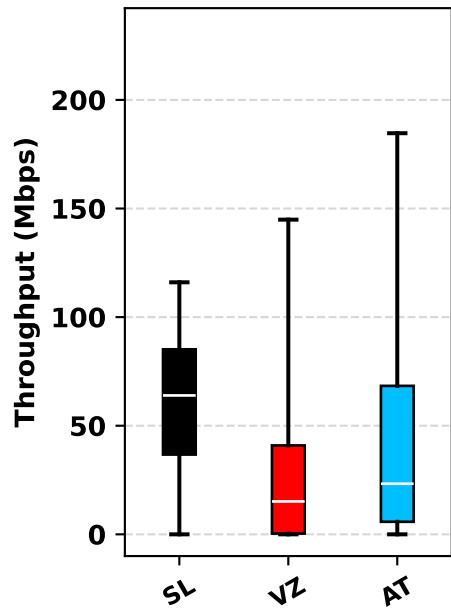
Single Flow
