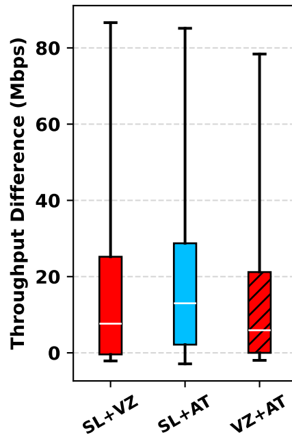
MPTCP – Max
