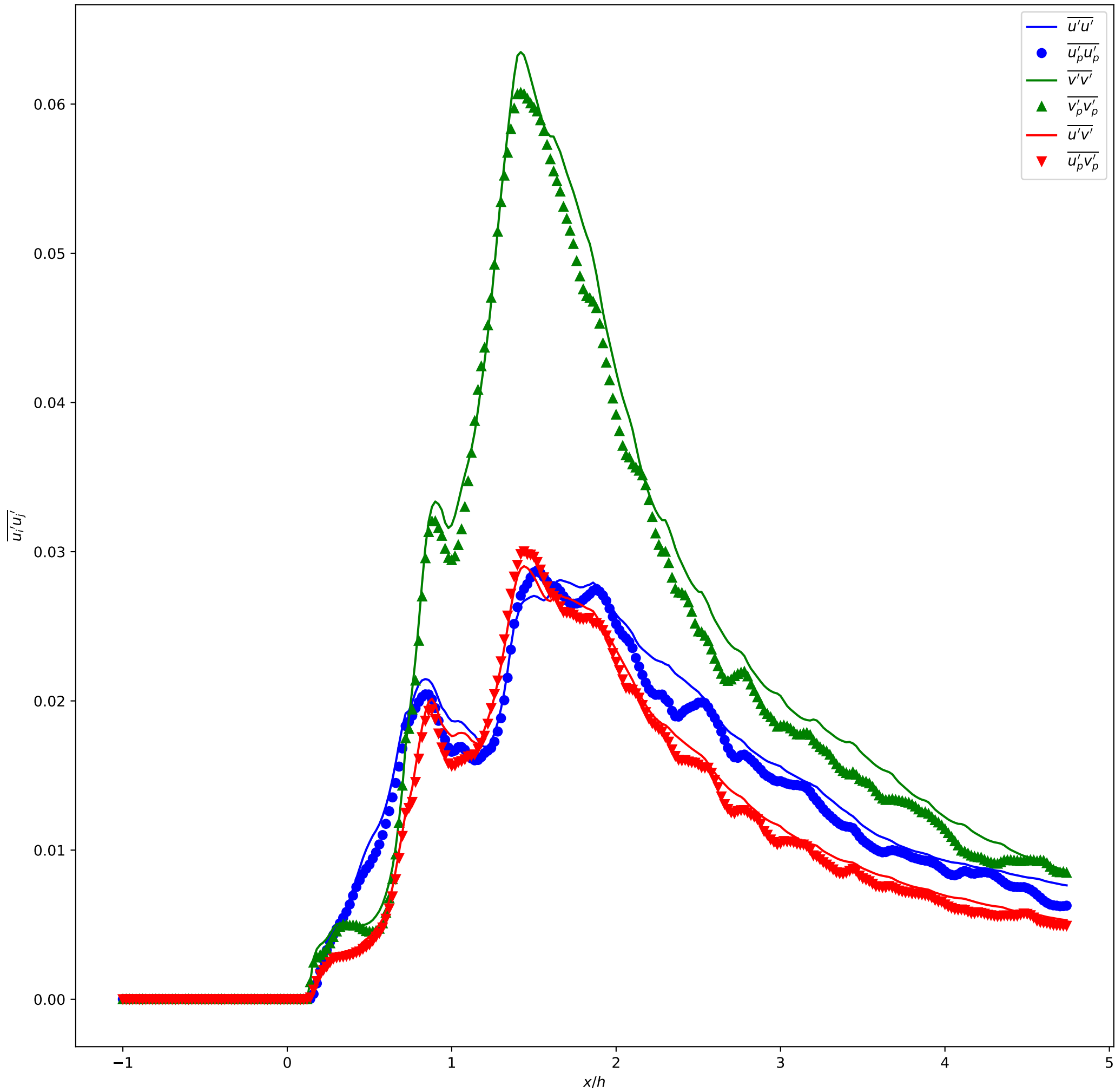
Reynolds Stress Components
