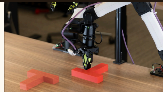
Push T
