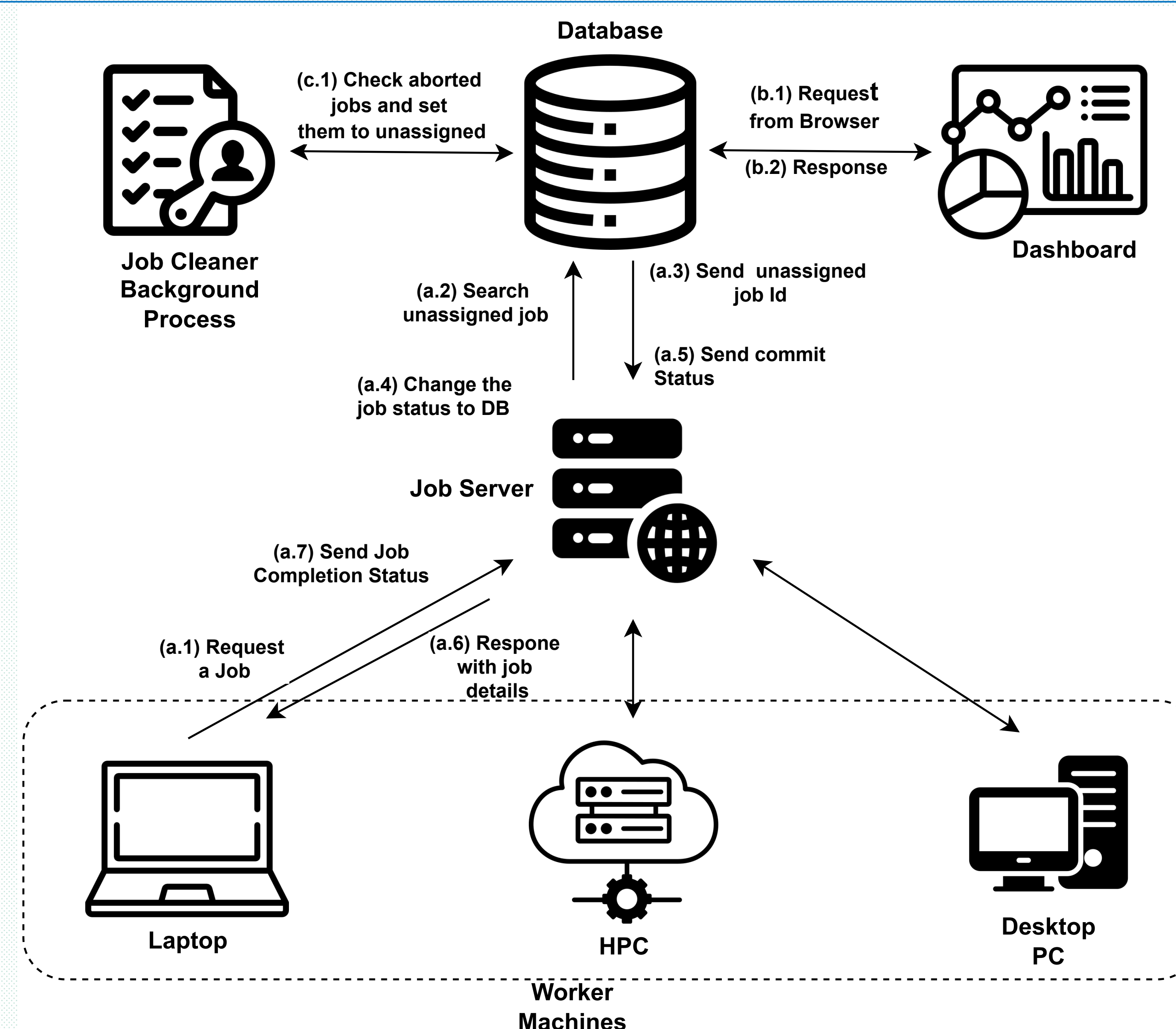
Figure: System architecture and job flow of the DART framework. Flows: (a.x) is the main job assignment and execution flow throughout the system; (b.x) is the information flow between database and dashboard; (c.x) is the handles fault tolerance of system between job cleaner and database.
