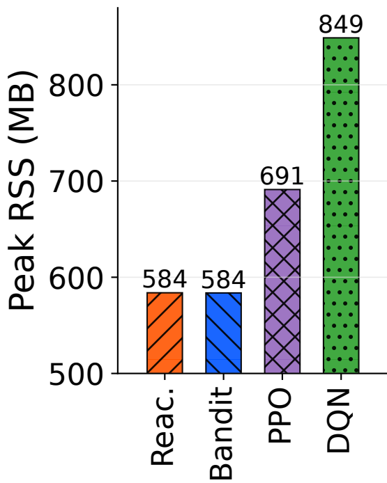
Peak RSS
