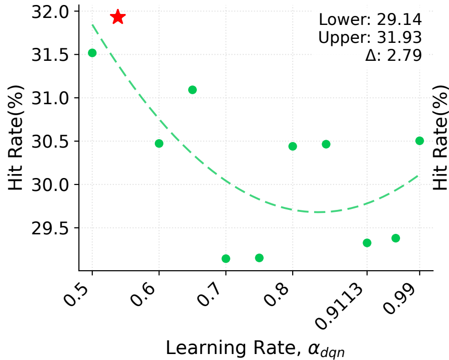
Spec. (DQN)
