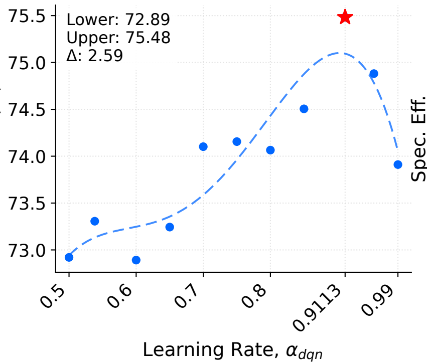
Spec.+Reac. (DQN)
