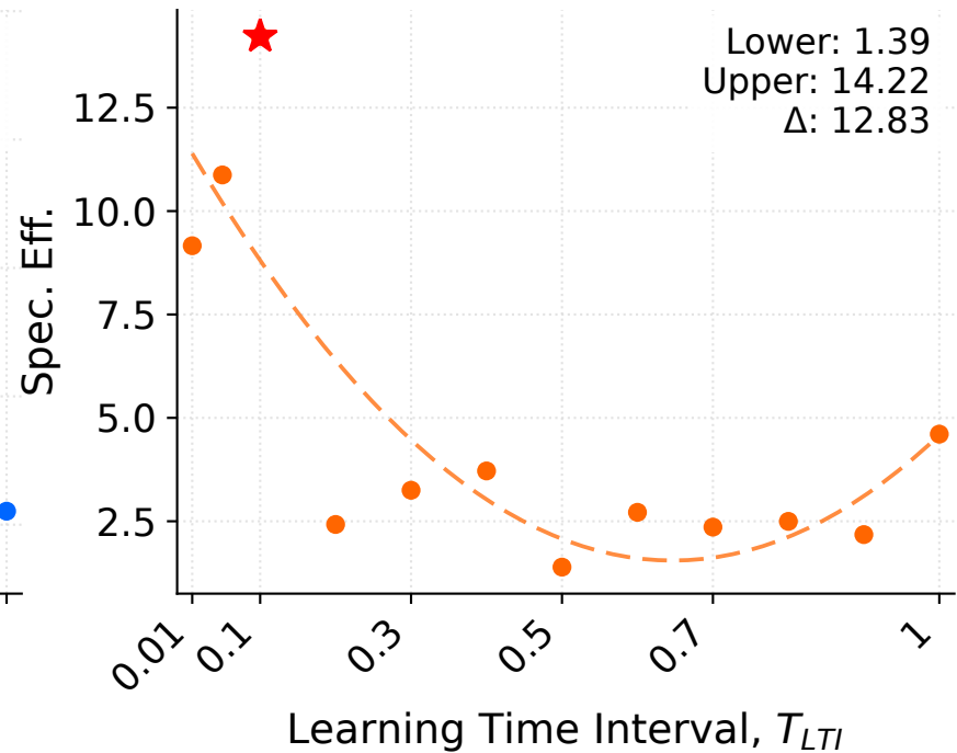
Spec. Eff. (Bandit)
