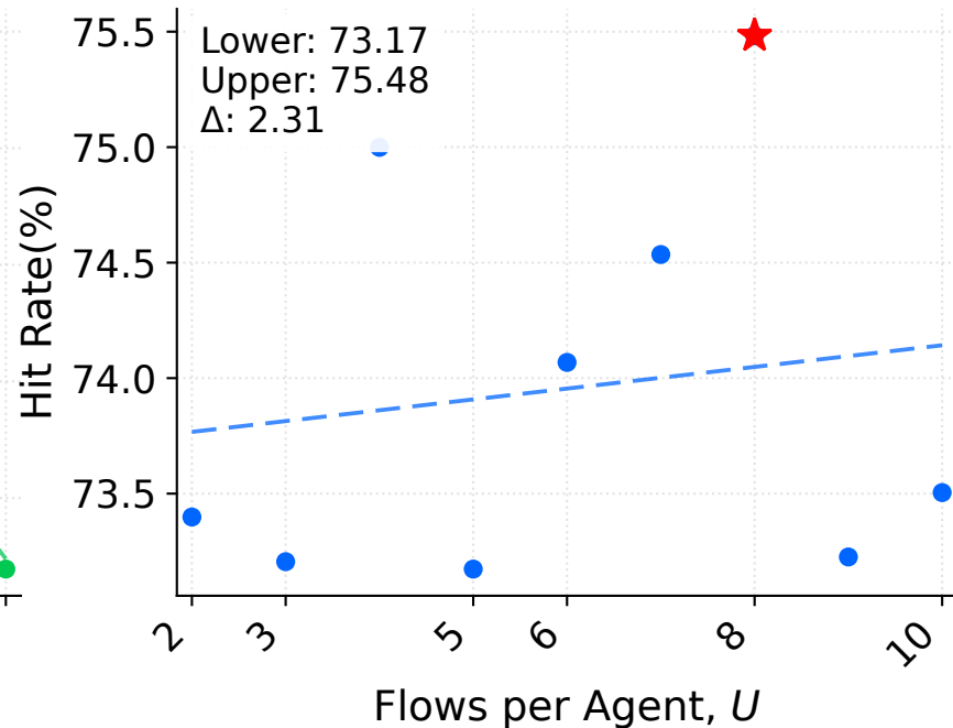
Spec.+Reac. (DQN)
