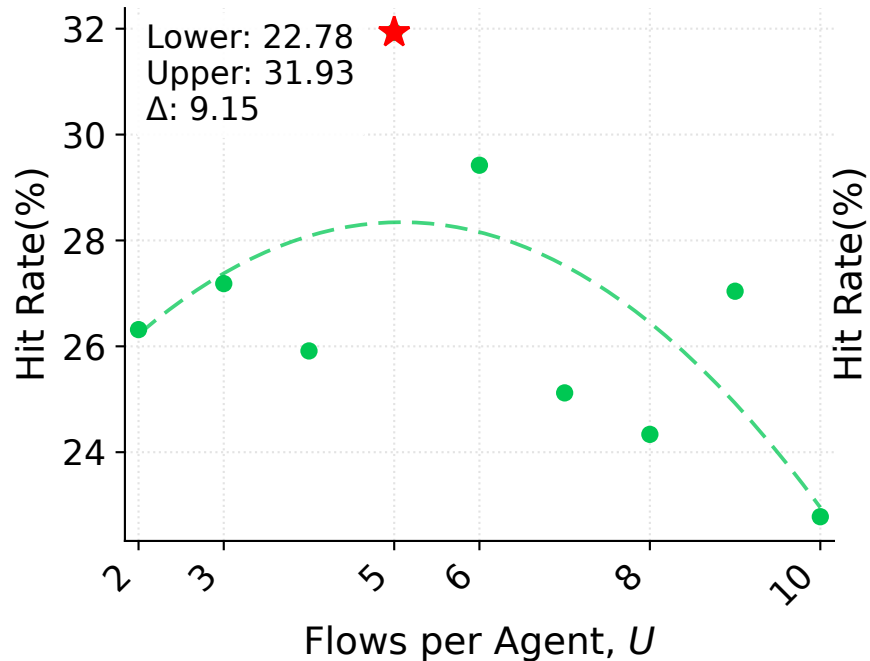
Spec. (DQN)
