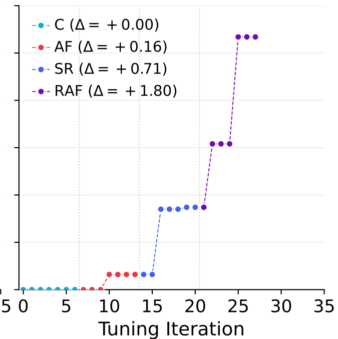
Speculation Efficiency Bandit(Trace)
