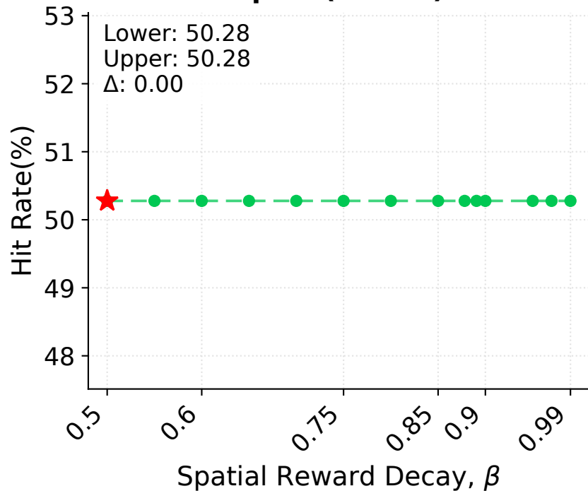
Spec. (Bandit)
