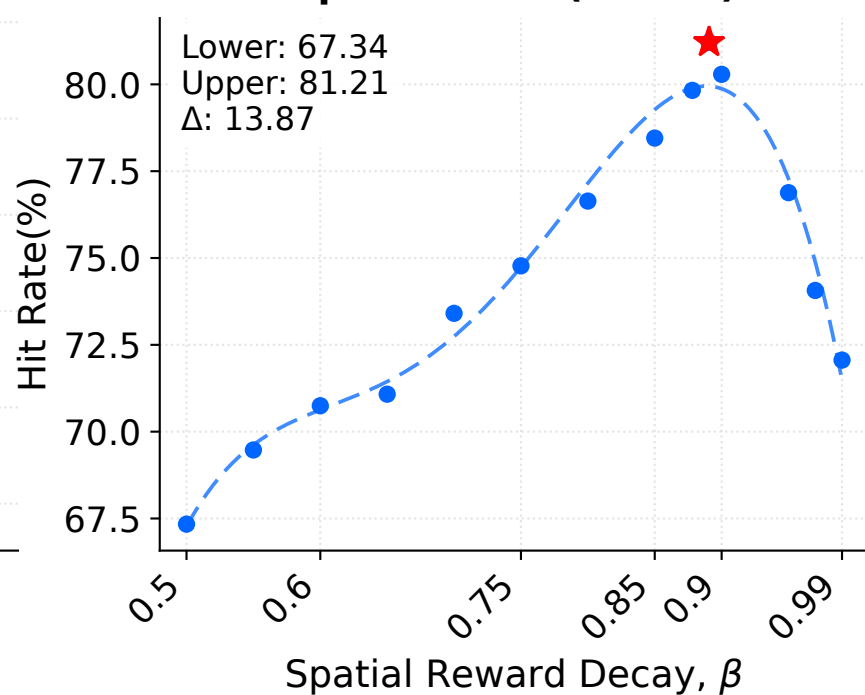
Spec.+Reac. (Bandit)
