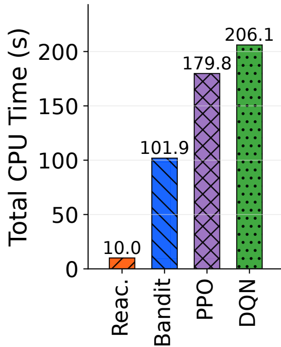
Total CPU Time
