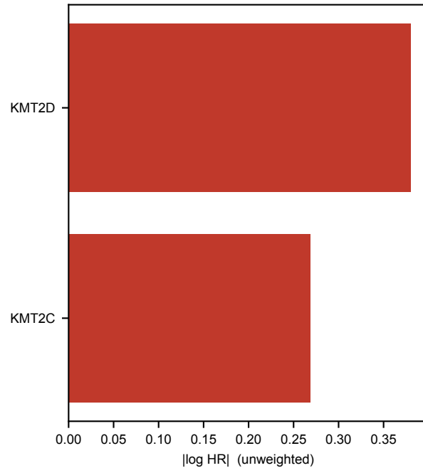
Chromatin_sv_hit
