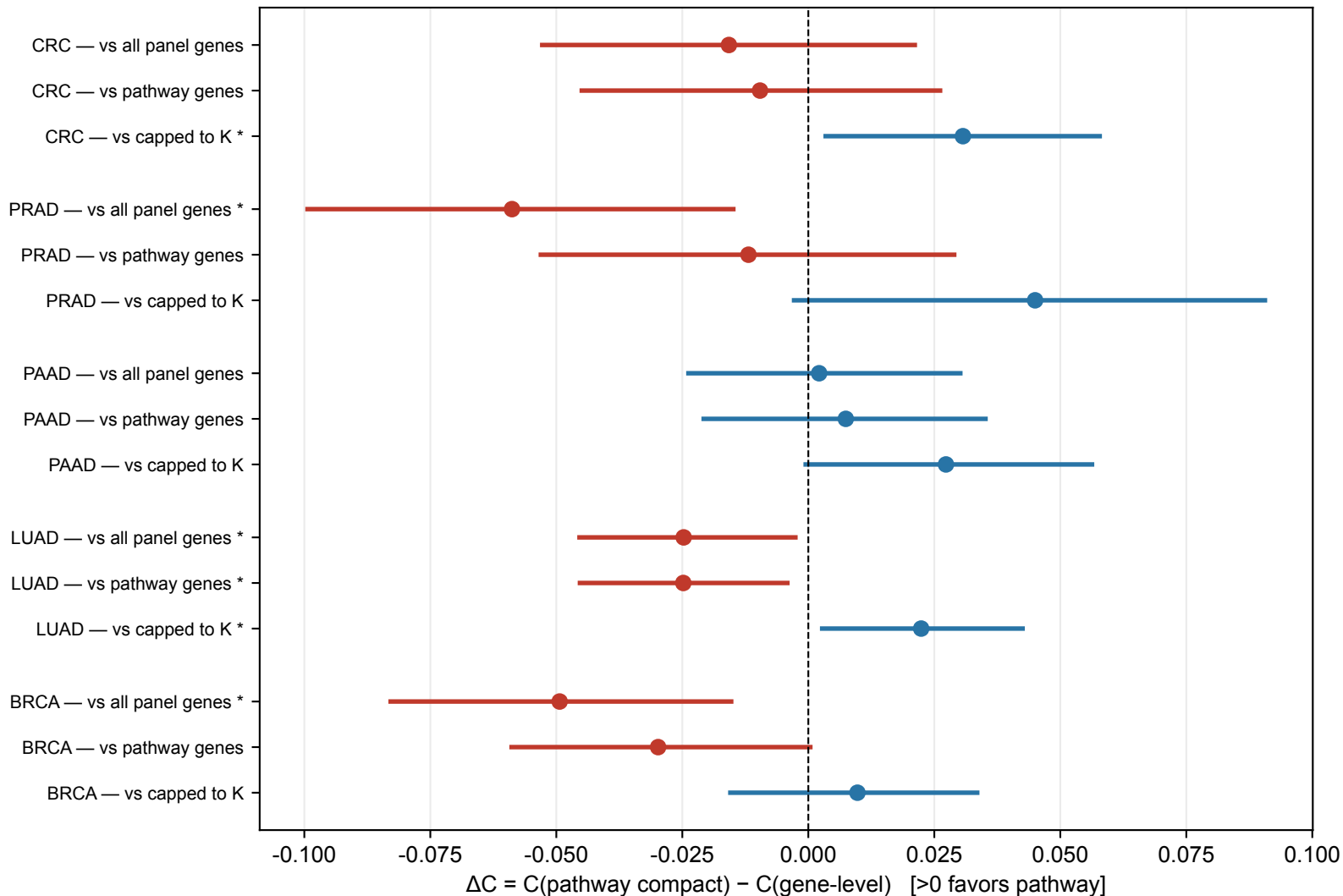
Paired test-set bootstrap \Delta C (1000 resamples); * p < 0.05
