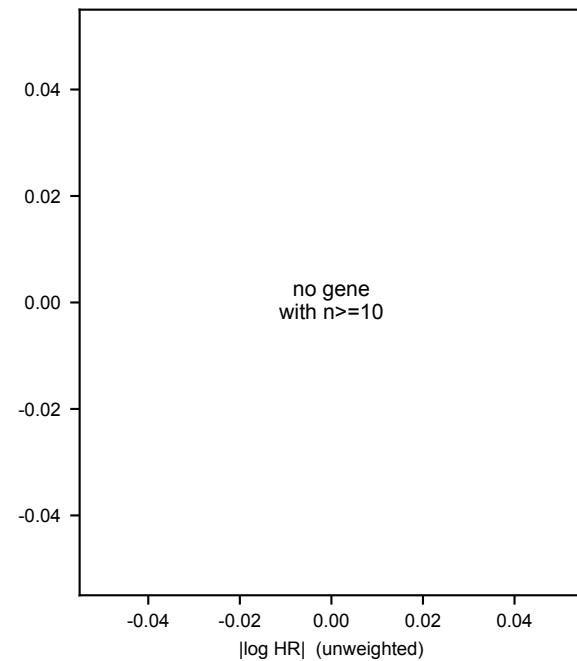
TGF_Beta_amp_hit
