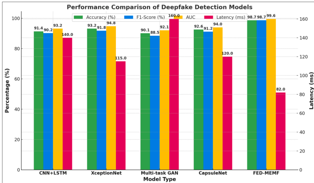
Fig. 3. Comparative analysis of various deepfake detection models.
