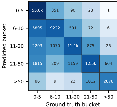
Memory buckets
