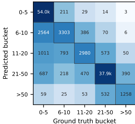
Wall-time buckets
