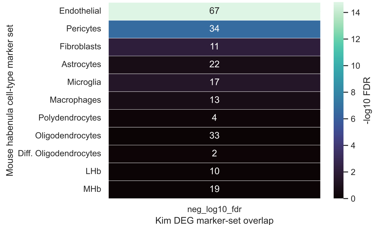
Fisher enrichment of Kim DEGs in cell-type markers
