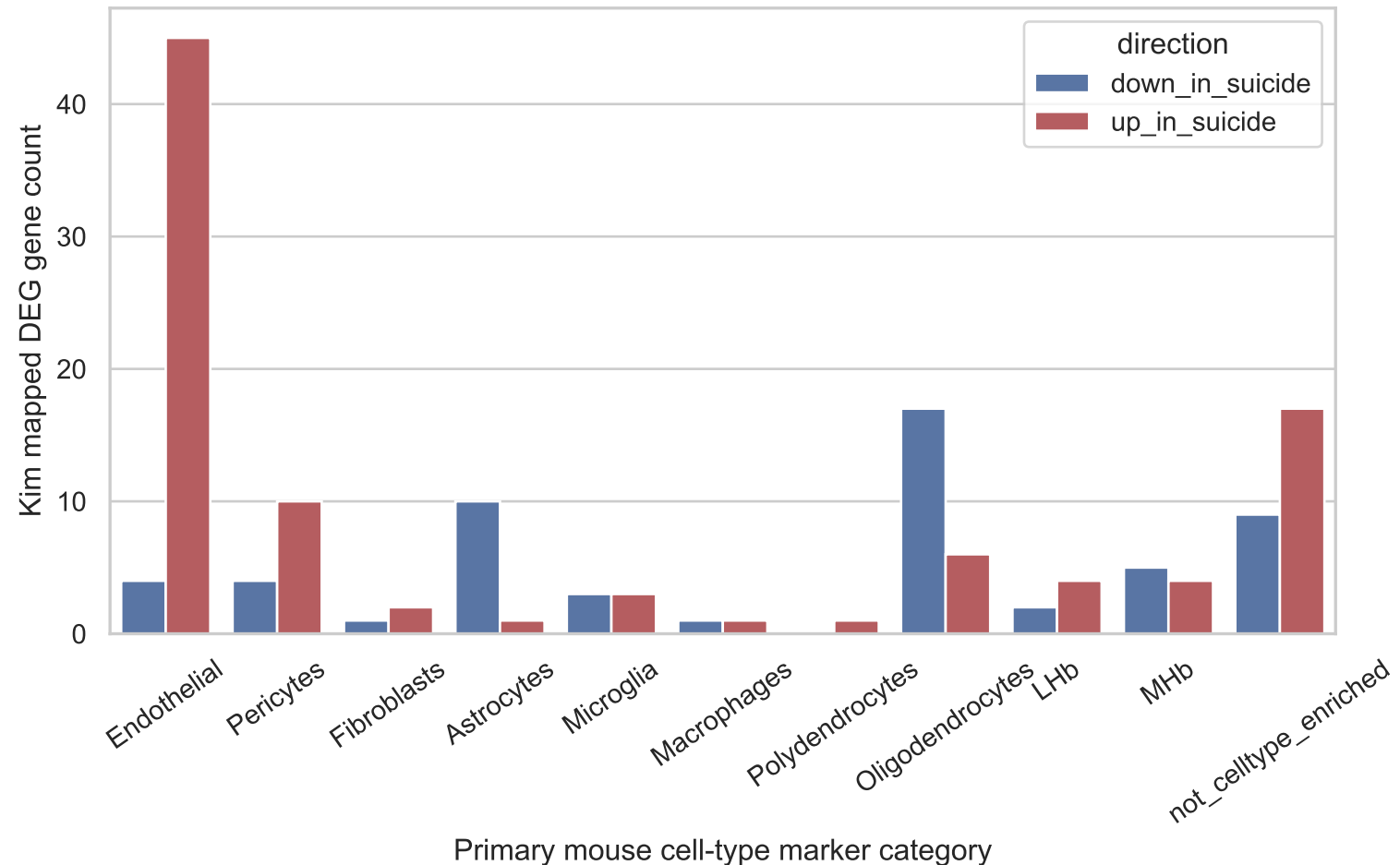
Kim suicide Hb DEGs categorized by mouse habenula cell-type enrichment
