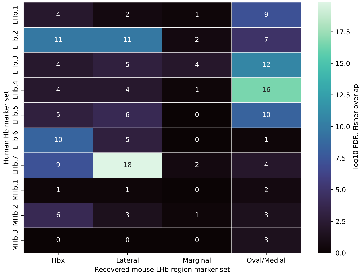
Analysis A: marker overlap using recovered LHb regions
