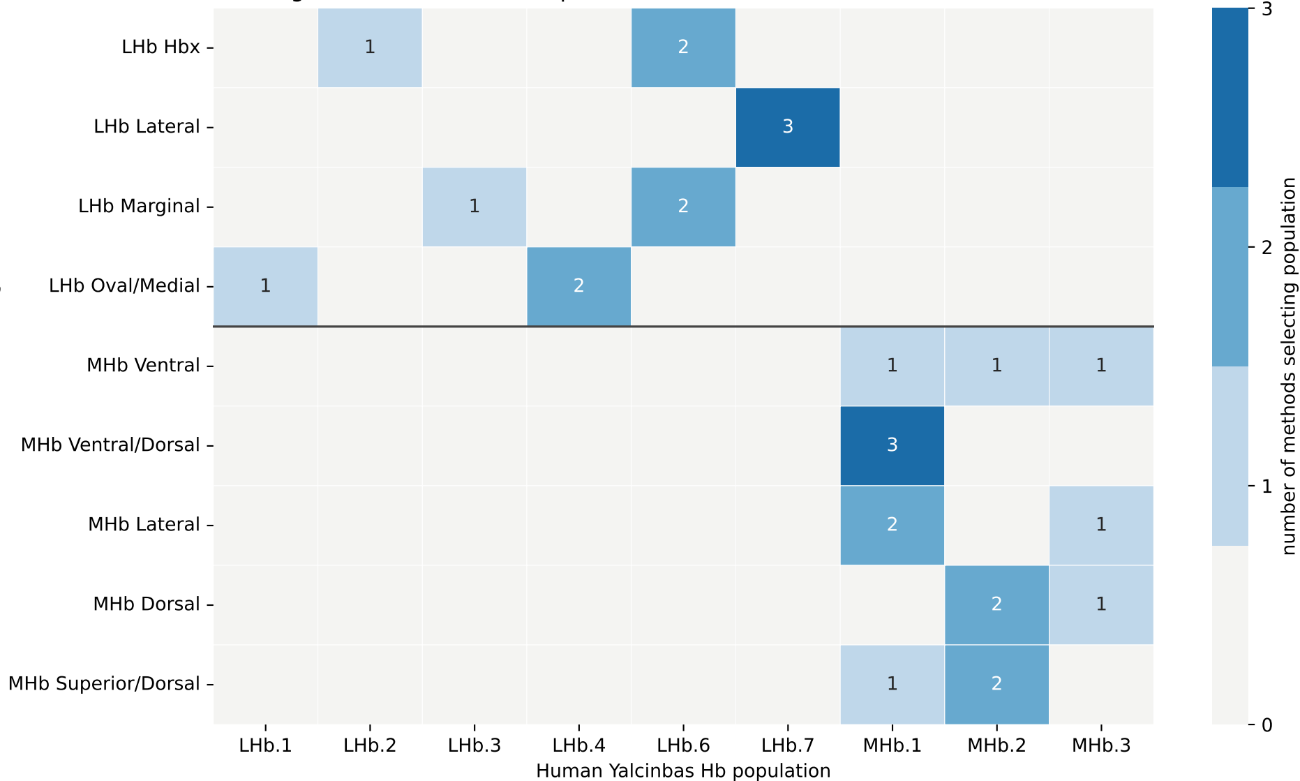
Agreement Across Overlap, Module Score, And Rank-Correlation Matches
