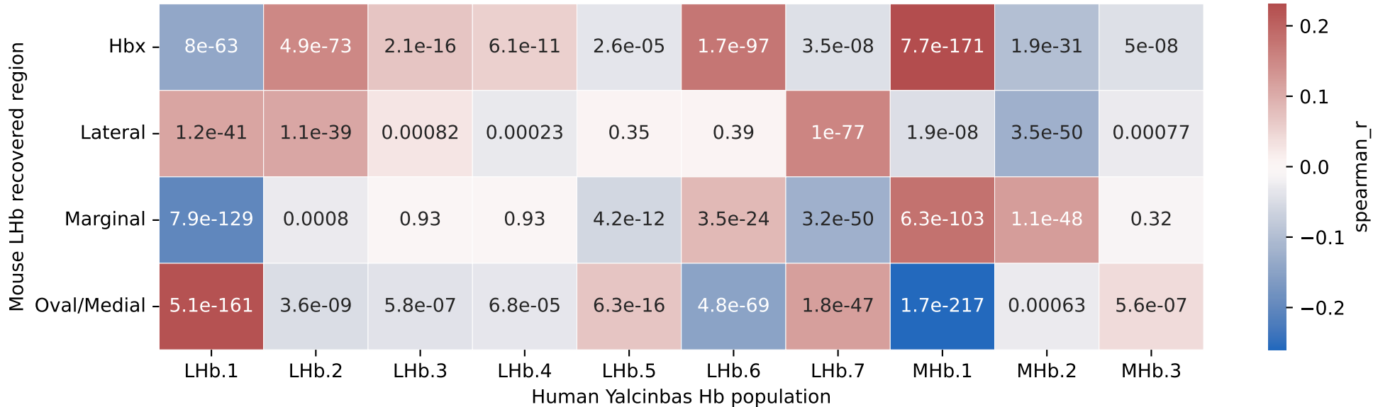
LHb: threshold-free human-vs-mouse marker score Spearman correlation
