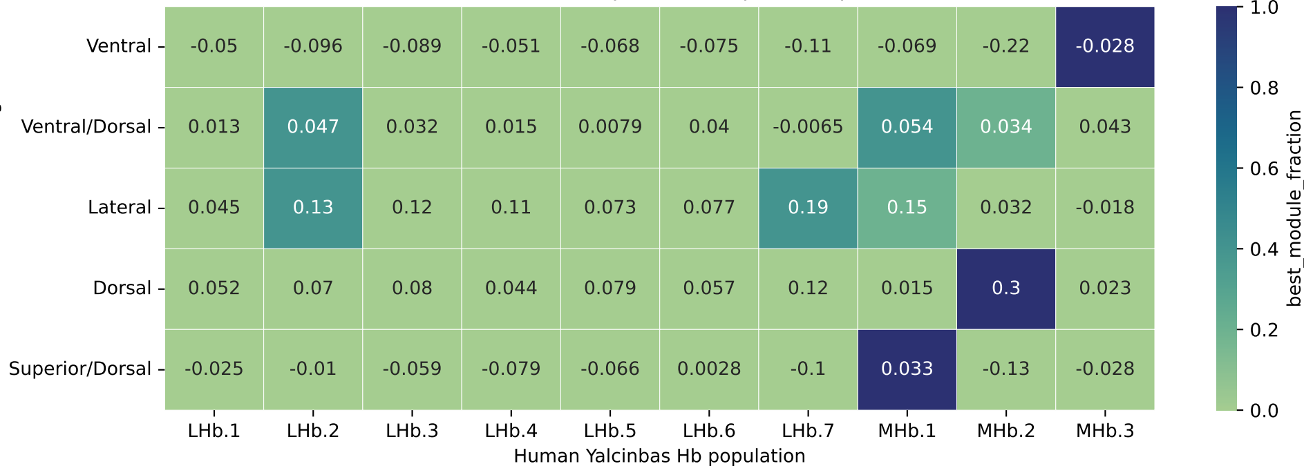
MHb: fraction of module depths where pair is top module score
