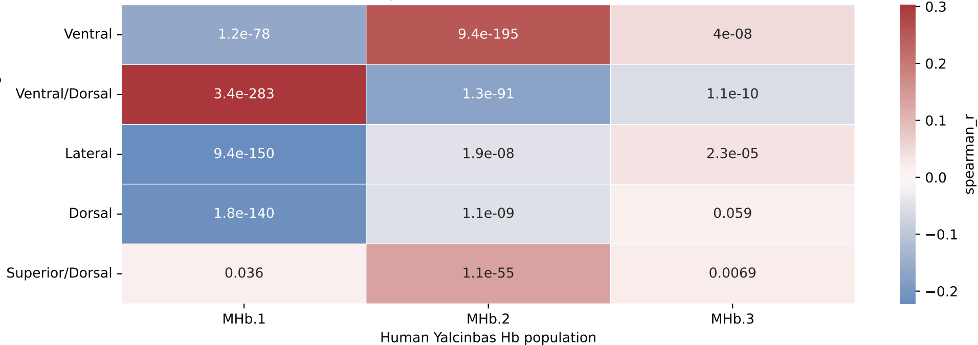
MHb: same-compartment threshold-free rank correlation
