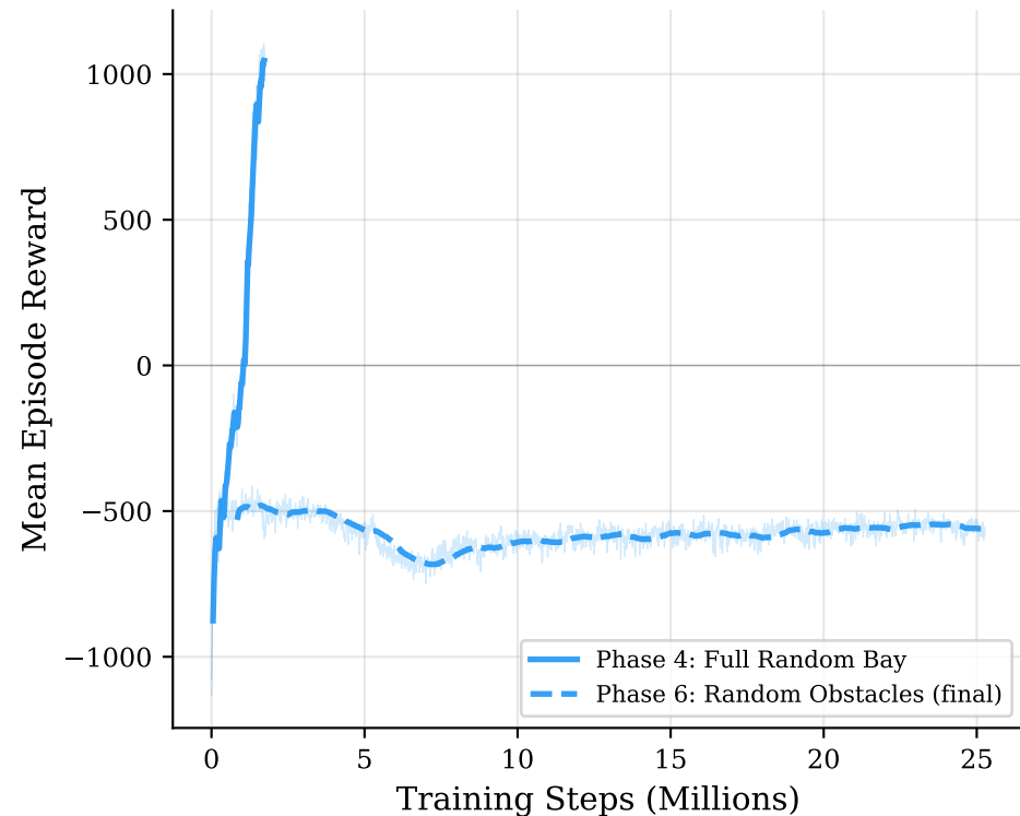
Original RL (reference) Reward Learning Curves
