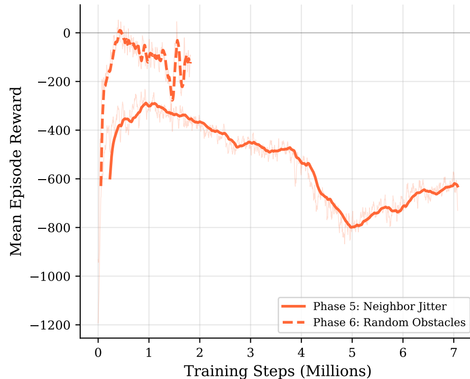
ChronosCar (1/28 scale) Reward Learning Curves
