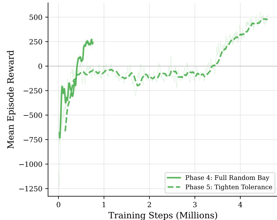
New Car (encoder) Reward Learning Curves
