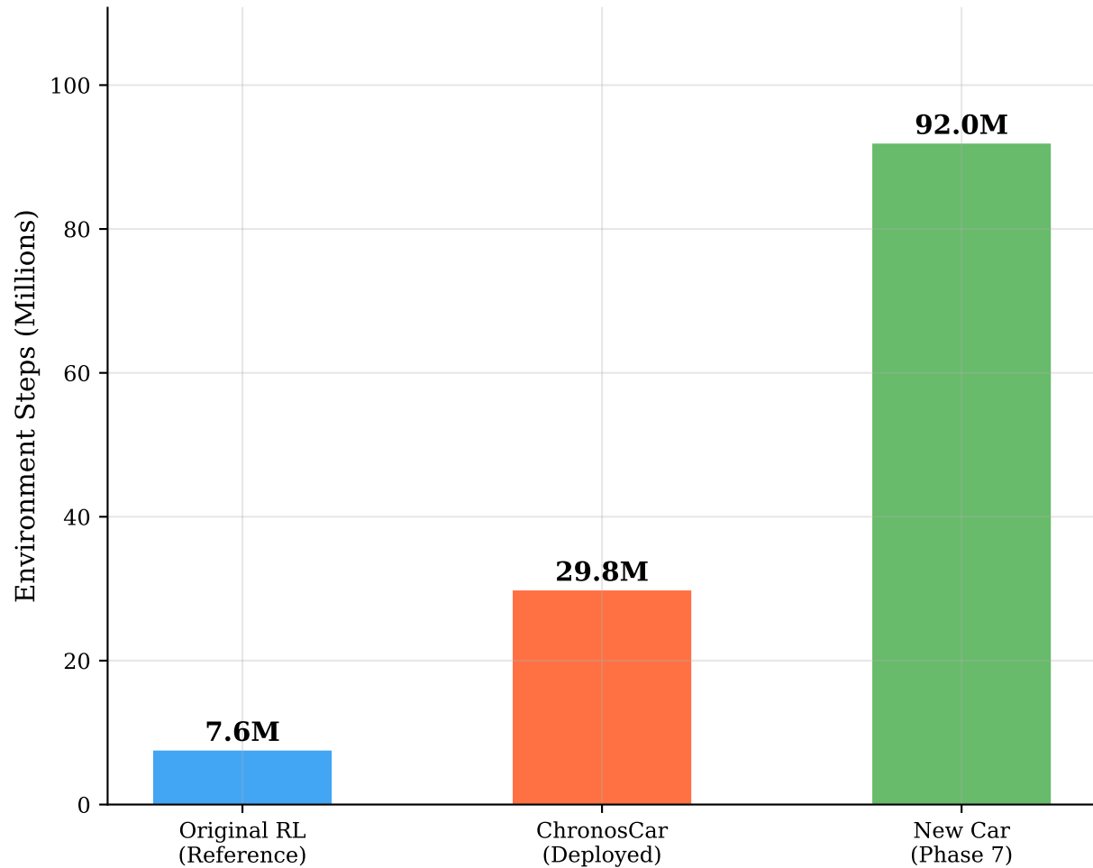
Total Training Steps (Sum across all curriculum phases)
