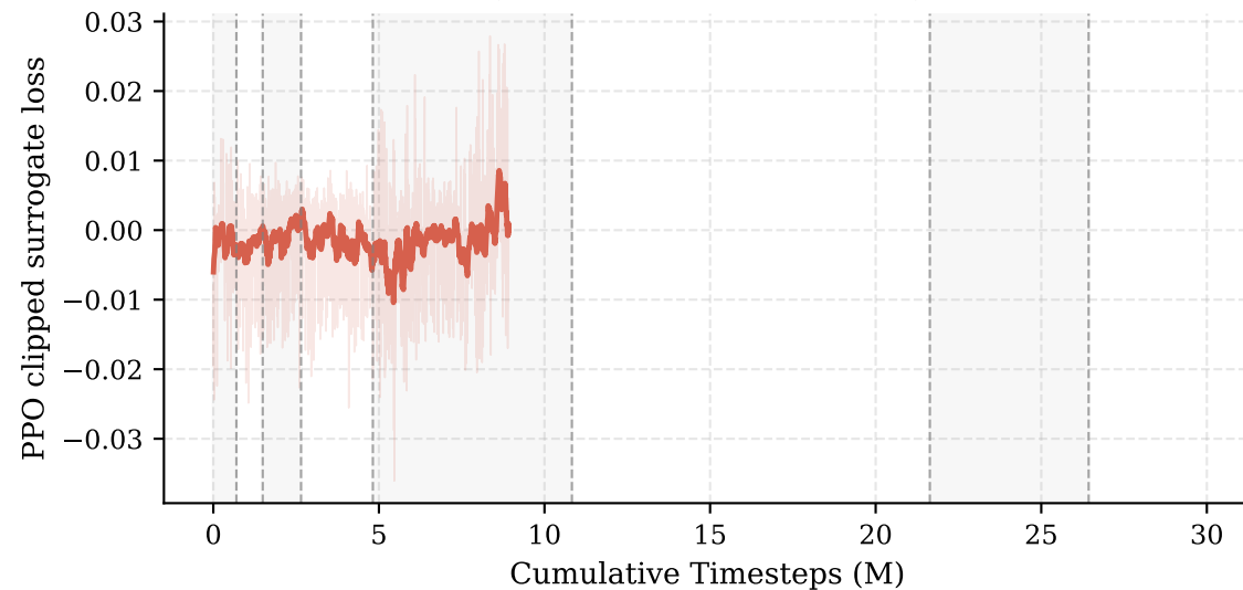
Policy Loss (Should decrease then stabilize)
