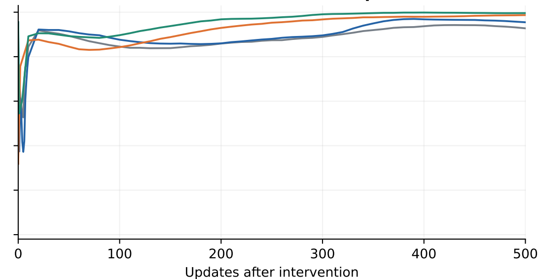
Seed 0, first 500 resumed updates
