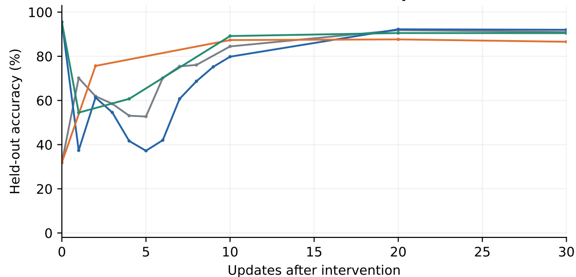
Seed 0, first 30 resumed updates
