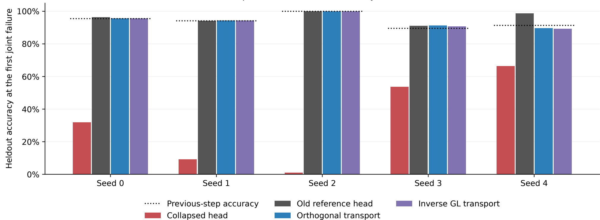
Previous-step readouts restore accuracy across five seeds
