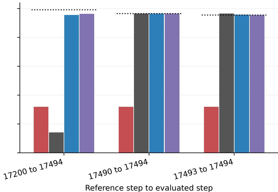
Seed 0
