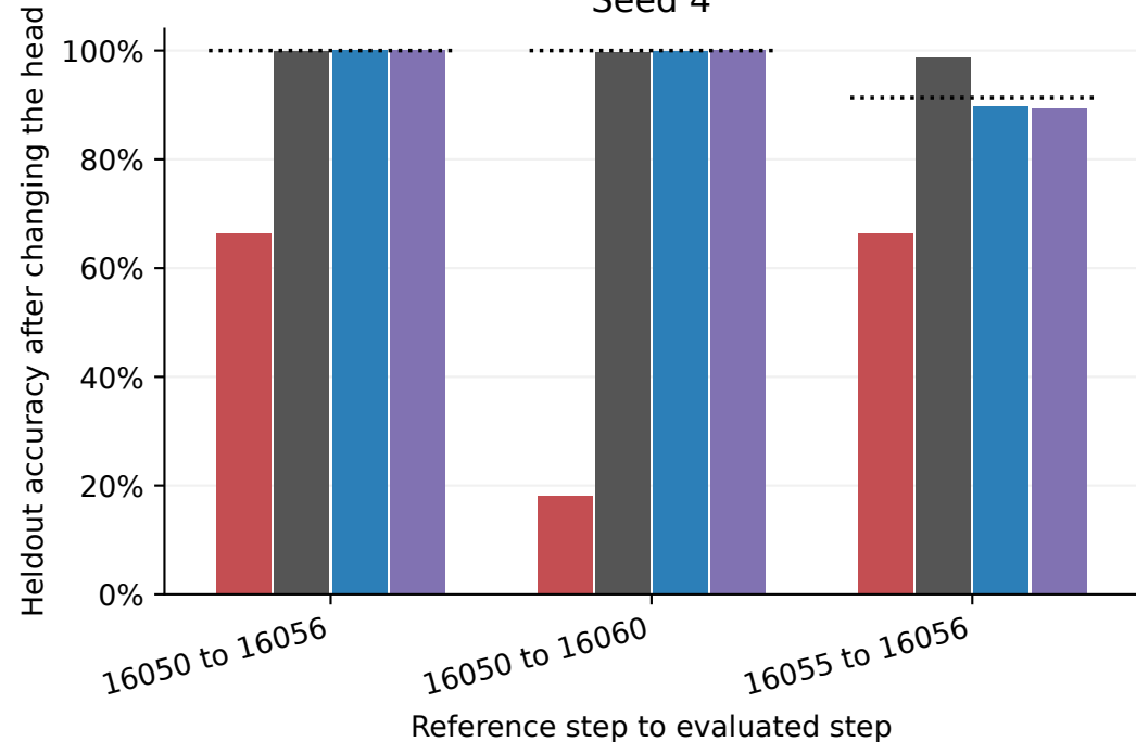
Seed 4
