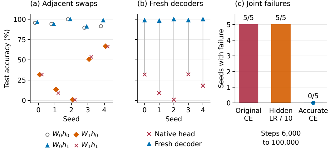
Figure 3: Follow-ups on five selected unnormalized trajectories; panels reuse seeds. (a) Adjacent swaps: 0/1 denote states before/after the captured update. The old head retains accuracy on new features; the new head lowers accuracy on old features. (b) Training-only decoders recover 98.20–100% at collapsed snapshots; seeds 3 and 4 use later snapshots than (a). (c) Joint train/test failures below 90%: original CE 5/5, hidden LR/10 5/5, accurate CE 0/5. Continuations share step-6,000 sources and end at 100,000. Binary incidence compares mixed original monitoring (failures captured before 30,000) with complete joint-event detection in both continuations (Appendix J).
