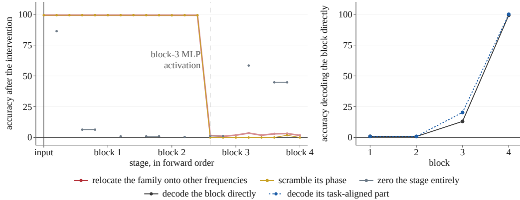
Figure 7: Depth-4 Muon at step 53,000. Left: the reported stage-intervention realization. Relocation and phase scrambling first cause a large drop at the block-3 MLP activation. The two stochastic curves use replicate 4 of five and illustrate sensitivity; individual later-stage outcomes vary across perturbations. Zeroing the earlier block-2 and block-3 attention writes also destroys accuracy, despite their low sensitivity to these Fourier perturbations. Right: direct decoding through the final unembedding, using each post-block residual or its addition-filtered component. Both reach high accuracy only at the final block.
