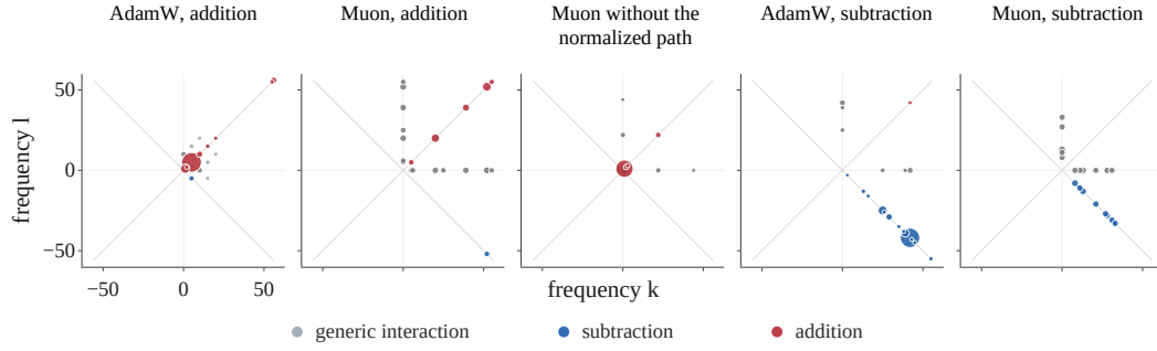
Figure 6: The twenty highest-power conjugate pairs of the final residual at converged checkpoints, on the mode grid, sized by share of non-constant power; grey lines mark l = k and l = -k . AdamW places 80.1% of non-constant power on a single pair of the family the task selects; Muon’s strongest pair carries 7.9%, with the rest spread across the family and beyond it; ablating the normalized path returns the strongest pair to 58.9%. Between the addition and subtraction panels the occupied line moves from one diagonal to the other.
