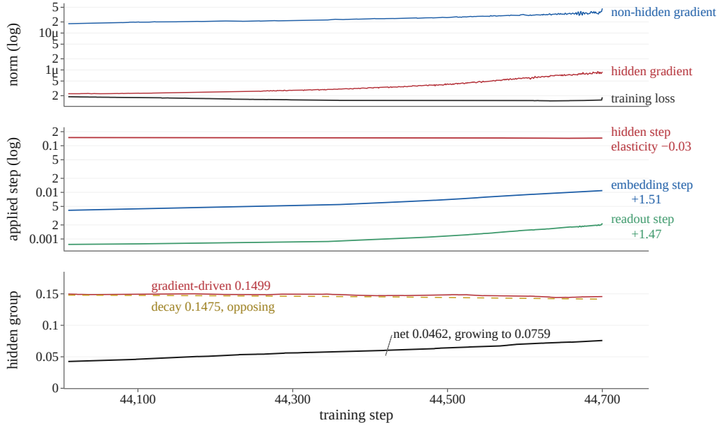
Figure 5: Every-step measurements over 691 updates before a collapse. Top: loss and gradient norms in the quiet window. Middle: gradient-driven applied steps and log-log slopes against the hidden gradient norm for Muon and the combined non-hidden norm for both AdamW groups. Bottom: hidden step and decay magnitudes differ by under 2% at step 44,100. Their vector sum is smaller and grows by 64% from step 44,100 to 44,700 while the gradient-driven step changes little.
