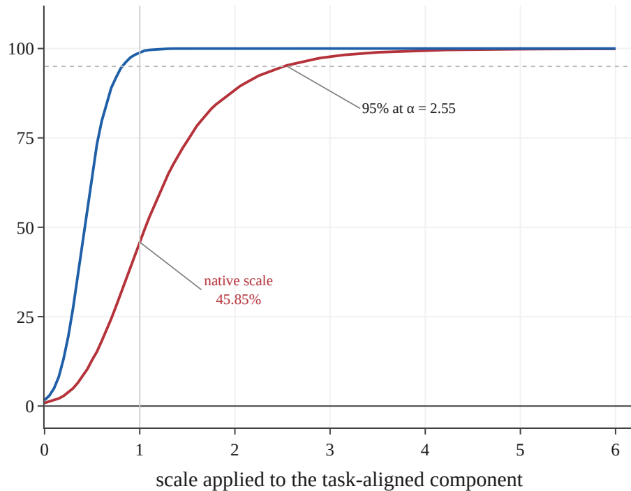
accuracy of the full model
