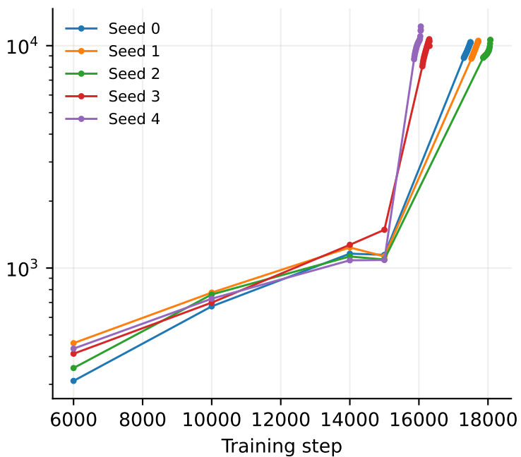
Feature mean norm
