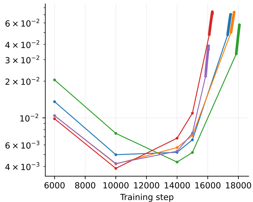
Classifier mean norm
