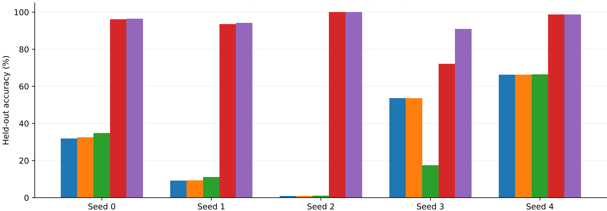
Exact next-step interventions at five captured joint failures
