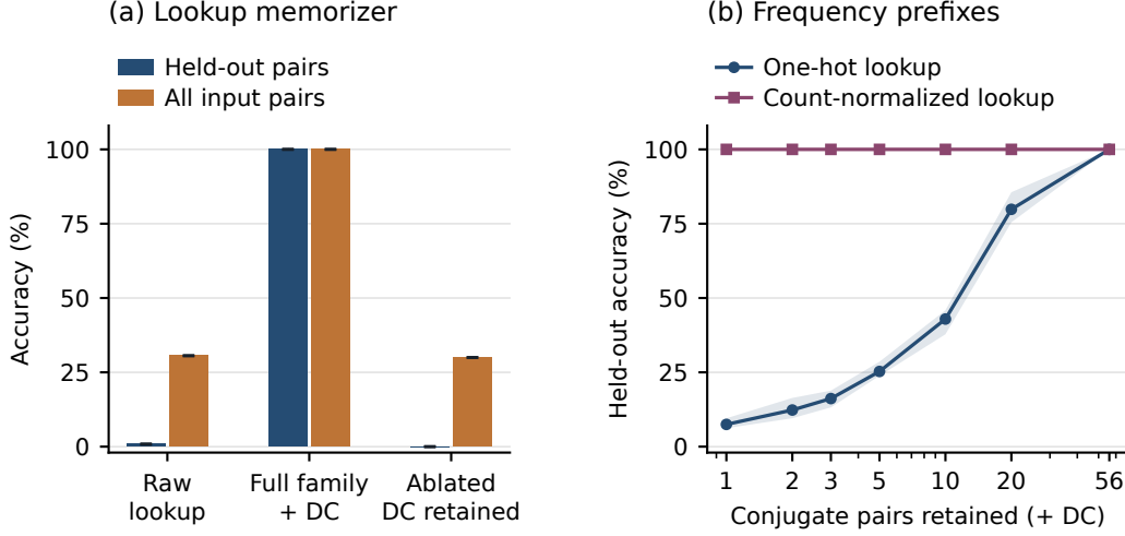
Figure 9: Task structure supplied by Fourier filtering at p = 113 . (a) The lookup memorizes the 3,830 training answers and returns zero on the 8,939 held-out inputs. Full-family filtering with DC gives 100% accuracy. Family ablation retains DC and yields 0% held-out accuracy and 29.99% full-grid accuracy. Bars show means over five splits; whiskers span their range. (b) Training-count normalization allows any one diagonal conjugate pair plus DC to classify every input correctly. The ordinary lookup’s pair powers are mathematically tied; its prefixes use increasing frequency as a fixed tie break. Lines show means and shading spans the seed range.
