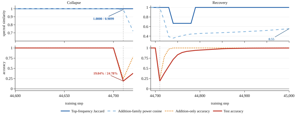
Figure 1: A model and its filtered pathway failing, at ten-step evaluation resolution. Left: test accuracy falls from 100% to 19.04% and addition-filtered accuracy to 24.78%. The five dominant addition-frequency pairs are unchanged (Jaccard 1.0000), and power over all 56 addition pairs retains cosine similarity 0.9899. Right: accuracy returns to 99.90% within 300 steps, with power cosine 0.55. The same five pairs remain dominant, with a different allocation of power. The addition family consists of the non-constant (k, k) modes of the final residual’s operand-grid Fourier transform; accuracy filters also retain the constant mode.
