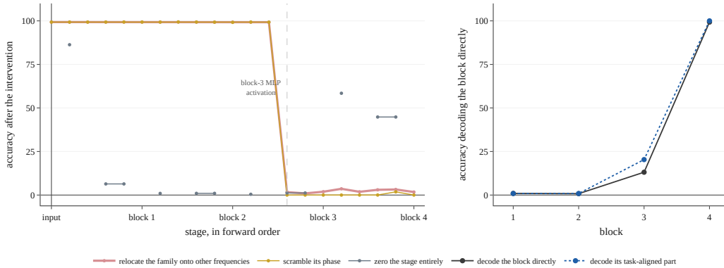
Figure 7: Depth-4 Muon at step 53,000. Left: the reported stage-intervention realization. Relocation and phase scrambling first cause a large drop at the block-3 MLP activation. The two stochastic curves use replicate 4 of five and illustrate sensitivity; individual later-stage outcomes vary across perturbations. Zeroing the earlier block-2 and block-3 attention writes also destroys accuracy, despite their low sensitivity to these Fourier perturbations. Right: direct decoding through the final unembedding, using each post-block residual or its addition-filtered component. Both reach high accuracy only at the final block.
