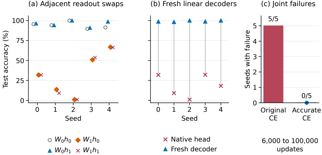
Figure 3: Follow-ups on five selected unnormalized trajectories. (a) Adjacent swaps: subscripts 0 and 1 denote states before and after the captured update. The old head retains accuracy on updated features; the new head sharply lowers accuracy on old features. (b) Training-only decoders recover 98.20–100% at collapsed snapshots; seeds 3 and 4 use later snapshots than (a). (c) Every original trajectory has a captured joint train/test failure below 90%; accurate CE from the matched step-6,000 state yields 0/5 through 100,000. Original failures were captured before step 30,000. Panels reuse seeds. Counts report binary incidence under mixed original monitoring and complete joint-event detection in corrected branches (Appendix J).
