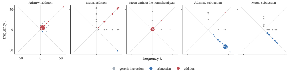
Figure 6: The twenty highest-power conjugate pairs of the final residual at converged checkpoints, on the mode grid, sized by share of non-constant power; grey lines mark l = k and l = -k . AdamW places 80.1% of non-constant power on a single pair of the family the task selects; Muon’s strongest pair carries 7.9%, with the rest spread across the family and beyond it; ablating the normalized path returns the strongest pair to 58.9%. Between the addition and subtraction panels the occupied line moves from one diagonal to the other.
