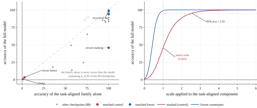
Figure 4: Left: task-aligned family accuracy (including the retained constant mode) against full-model accuracy over 98 checkpoints from the original studies, both evaluated through the current readout. Projection failure denotes low filtered accuracy; projection masking sits at the lower right, where the task-informed projection is accurate and the full model fails. The panel’s circuit labels refer to these operational outcomes. At 95 of 98 checkpoints the family alone is at least as accurate as the full model, and the three exceptions exceed it by under a point. Right: rescaling the non-constant task-aligned component of the masked checkpoint by \alpha , with the rest of the representation and the readout untouched.
