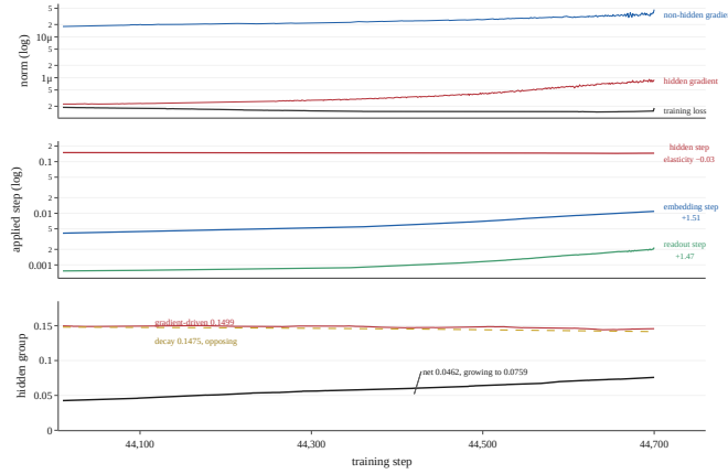
Figure 5: Every-step measurements over 691 updates before a collapse. Top: loss and gradient norms in the quiet window. Middle: gradient-driven applied steps and log-log slopes against the hidden gradient norm for Muon and the combined non-hidden norm for both AdamW groups. Bottom: hidden step and decay magnitudes differ by under 2% at step 44,100. Their vector sum is smaller and grows by 64% from step 44,100 to 44,700 while the gradient-driven step changes little.
