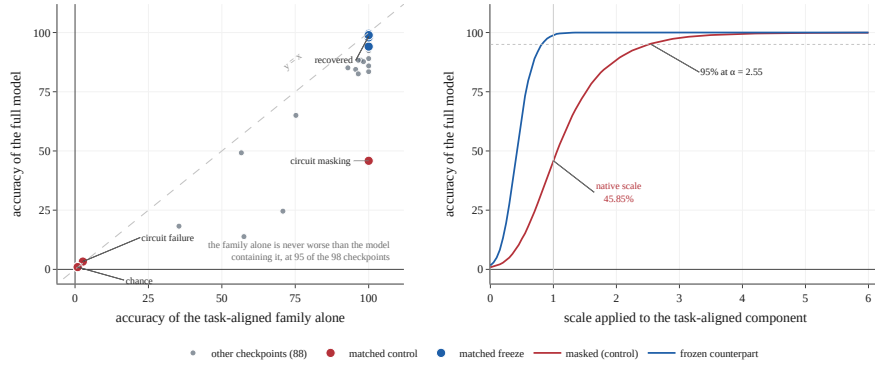
Figure 6: Left: task-aligned family accuracy (including the retained constant mode) against full-model accuracy over 98 checkpoints from the original studies, both evaluated through the current readout. Circuit failure denotes failure of this filtered pathway; circuit masking sits at the lower right, where the family solves the task and the model does not. At 95 of 98 checkpoints the family alone is at least as accurate as the full model, and the three exceptions exceed it by under a point. Right: rescaling the non-constant task-aligned component of the masked checkpoint by \alpha , with the rest of the representation and the readout untouched.
