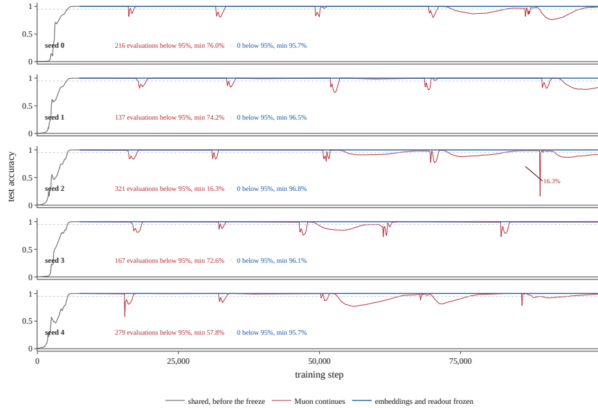
Figure 3: The intervention at five seeds. Before the freeze, the paired arms have identical logged metrics. One arm continues under ordinary Muon; the other holds embeddings and unembedding constant. The unfrozen arm falls below threshold 137 to 321 times per seed with minima as low as 16.27%; the frozen arm records none and never falls below 95.67%.
