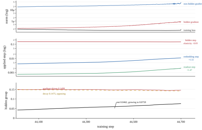
Figure 2: Every-step measurements over 691 updates before a collapse. Top: loss and gradient norms in the quiet window. Middle: gradient-driven applied steps and log-log slopes against the hidden gradient norm for Muon and the combined non-hidden norm for both AdamW groups. Bottom: hidden step and decay magnitudes differ by under 2% at step 44,100. Their vector sum is smaller and grows by 64% from step 44,100 to 44,700 while the gradient-driven step changes little.
