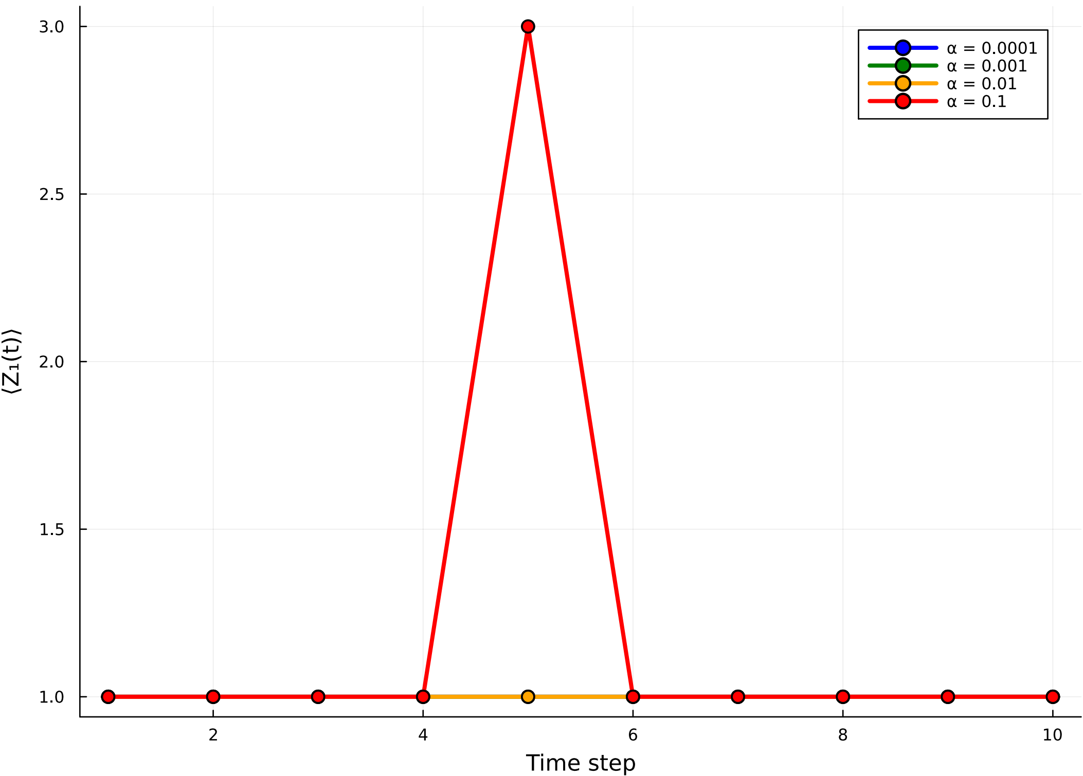
Correlation Function \langle Z_1(t) \rangle for Different \alpha Values (N=16)
