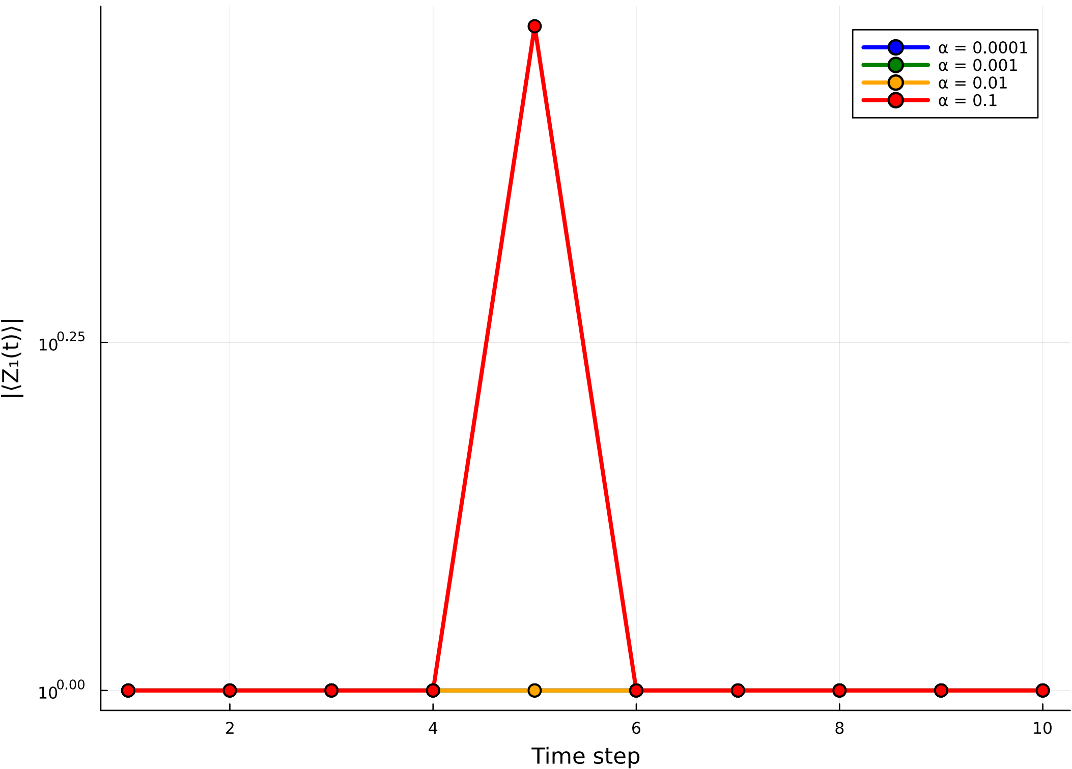
Correlation Function \langle Z_1(t) \rangle (Log Scale, N=16)
